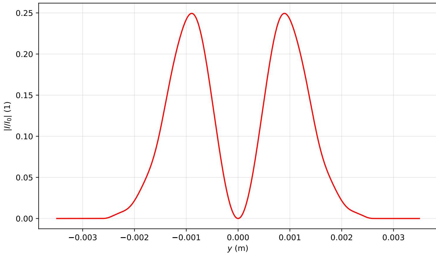
Intensity profile I(x=0, y, z=3.264)/I_0 , P_{in}=1.0P_{cr} , artificial time
